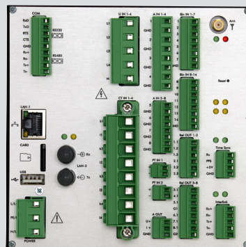
Abb. 2: Anschlüsse EPPE CX
